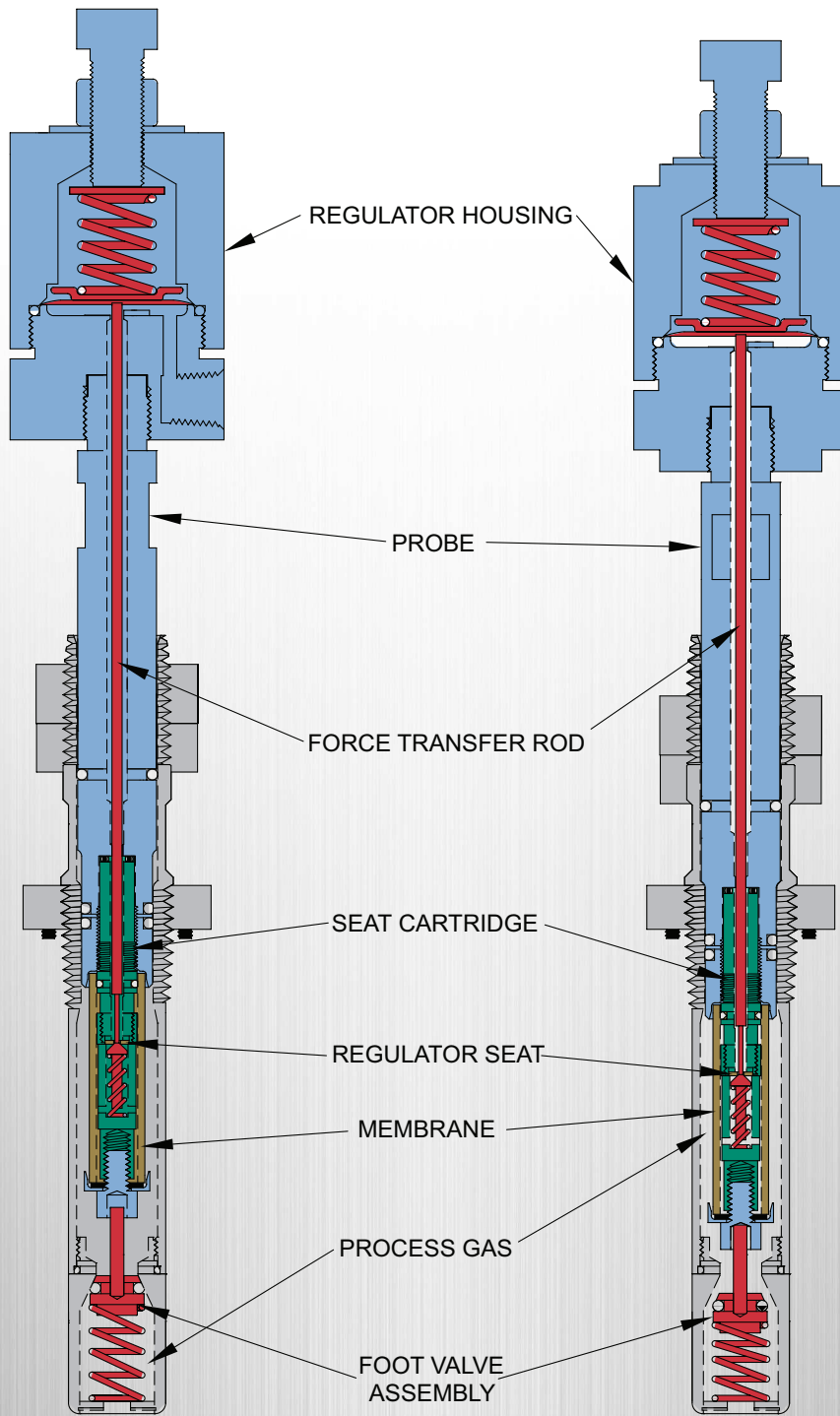
FOOT VALVE CLOSED
